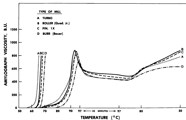
Fig. 2. Amylograph pasting curves obtained with rice flours ground from the same lot of rice on four different mills. Short curves, 20% slurries; full curves, 10% slurries.
