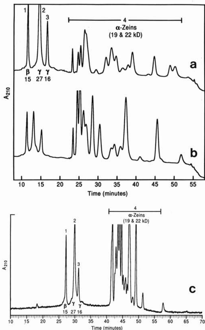
Fig. 4. Reversed phase high-performance liquid chromatograms of total zein fractions from (a) Kantz Flint maize, (b) Papago Flour maize, and (c) Ross Early Flint maize.
